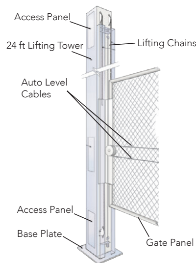
HydraLift™ Post
